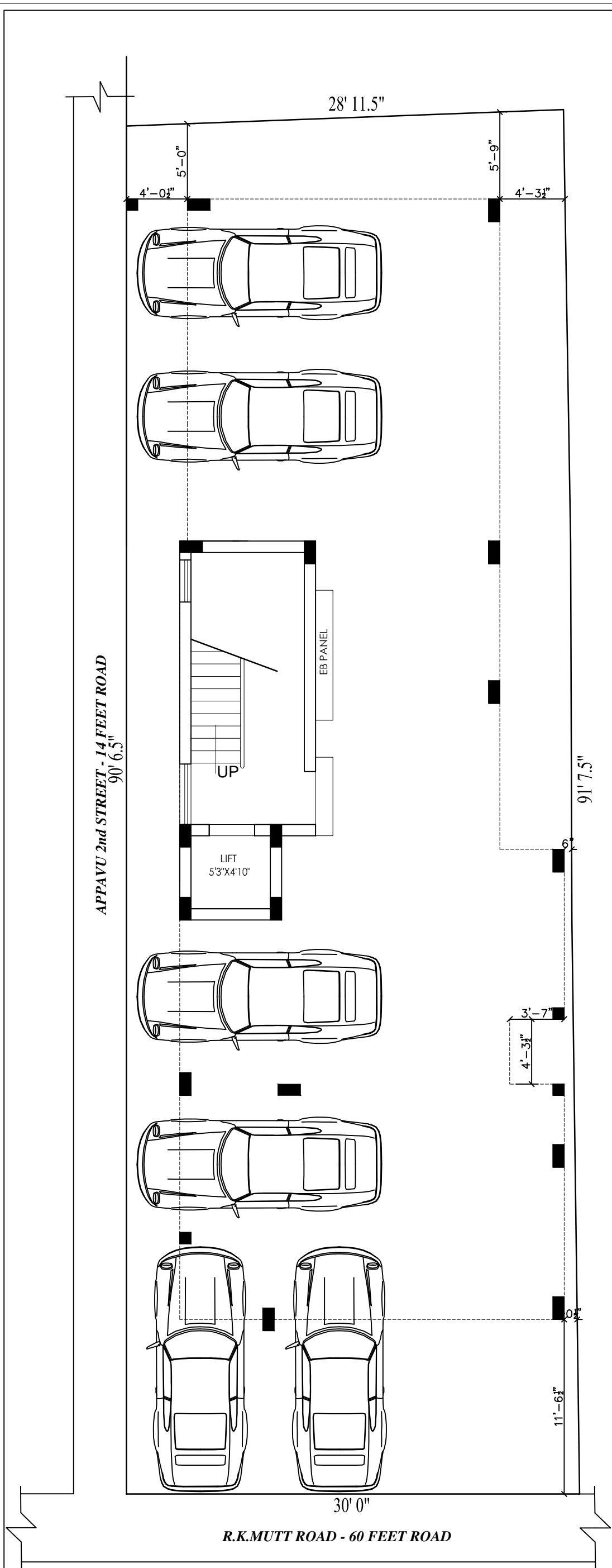
STILT FLOOR PLAN
